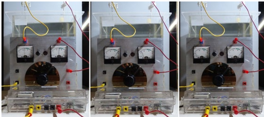
Figure 2: This shows the same instrument three times. Behind the instrument, the upper part of the tank filled with deionised water can be seen. The instrument itself contains two panel meters and a large dial plate housing a 1 million Ohm variable resistor, referred to as a potentiometer. In front of the instrument is the actual DC power supply providing 300 volts @ 50 micro ampere. The left panel meter represents the panel meter in series with the two submersed electrodes in the tank. The panel meter on the right is in series with the variable resistance. The picture on the far left shows an equal current in both panel meters at a half-scale deflection at 25 micro ampere, the picture in the middle shows a full scale deflection for the tank electrodes and the far right picture a maximum current of 50 micro ampere. Whenever current is biased in favour of one circuit, the other circuit will show less current. That is called current hugging. Since the variable resistance is 'Not' in the water, it can be said that "we are measuring the resistance of water without measuring the resistance of water". In this particular case the measured resistance proved to be 170,000 ohm approximately shared parallel between the current flow between the electrodes and the variable potentiometer.
