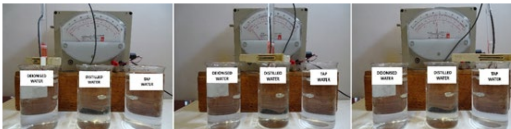
Figure 3: Analogue panel meter instrument in the background has a DC input resistance of 10,000 million Ohm and loads the water at just 1 volt DC. This loading is so small that a very high accuracy is obtained. There is almost no parallel resistance factor. Three jars are filled with deionised water in the jar on the left, commercially available distilled water in the jar in the middle and a jar filled with ordinary tap water on the right. The meter movement itself has a full scale deflection of 100 micro ampere and the readings obtained are 2.5 micro ampere for the deionised water, around 10 micro ampere for the distilled water (an 4 fold increase in conductivity) and a half scale deflection at around 50 micro ampere for the tap water. A 20 fold increase in conductivity. This instrument is also able to measure the conductivity of urine.
